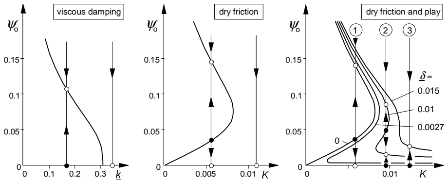
Fig. 6.26. Limit amplitudes as a function of damping for increasing number of non-linear elements: non-linear tyre, dry friction and play. ( V = 6.66 , \sigma = 3 , e = 0 , k^* = 0 ).
