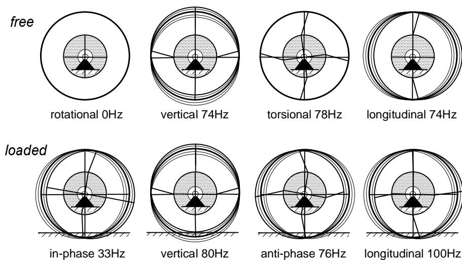
Fig. 9.39. Calculated in-plane vibrational modes of tyre/wheel system with axle fixed and tyre free or loaded on the drum surface with vertical load F_N = 4000\text{N} and at zero speed.
