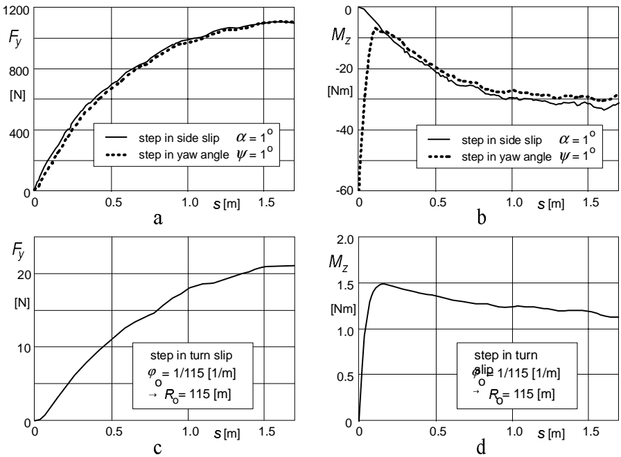
Fig. 5.12. Step response of side force F_y and aligning torque M_z to slip angle \alpha , yaw angle \psi and turn slip \phi ( \alpha = 0 ) as measured on a passenger car tyre at load F_z = 4 kN. Tests were conducted on the flat plank machine of TU-Delft. Turn slip results have been obtained by integration of the response to turn slip impulse = step yaw angle, and division by -R\psi . (From Higuchi, 1997).
