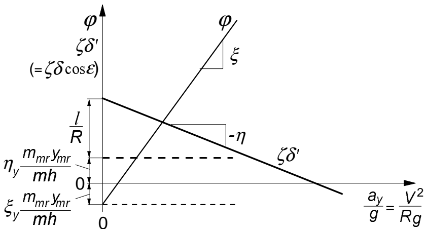
Fig. 10.16. The ground steer angle \delta' and the roll angle \phi due to path curvature l/R and c.g.lateral offset y_{mr} and the variation with lateral acceleration a_y .
