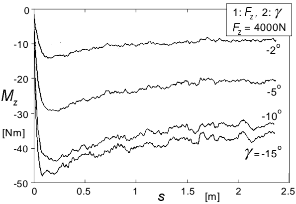
Fig. 7.11b. Moment response to step change in camber angle.
