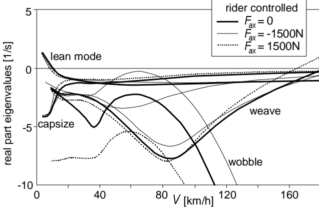
Fig. 10.13. The stability diagram with feed-back steer torque control of Fig.10.12 activated.
