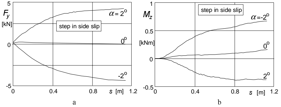
Fig. 5.11. Step response of side force F_y and aligning torque M_z to slip angle \alpha as measured on an aircraft tyre with vertical load F_z = 35 kN. (From Besselink, 2000; test data is provided by Michelin Aircraft Tyre Corporation).
