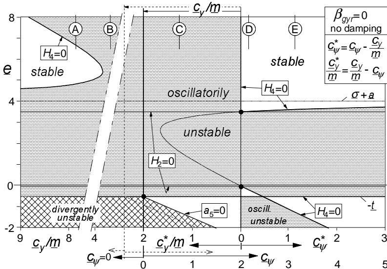
Fig. 6.10. Basic stability diagram according to conditions (6.46-48) for the fifth-order system without damping and gyroscopic coupling. The diagram hold in general, the case with c_y/m=2 is an example, note: m = 0.5 .
