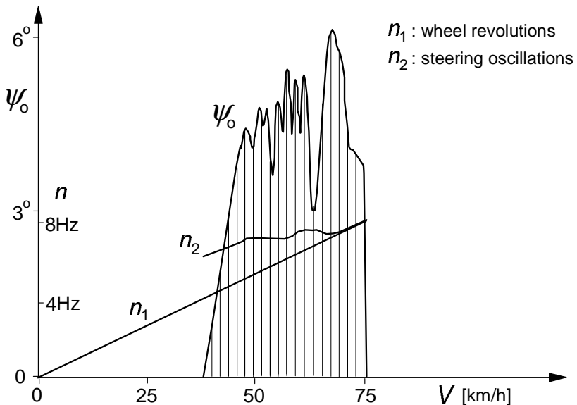
Fig. 6.31. Front wheel steer oscillation amplitude as a response to wheel unbalance as measured on a light truck. The speed is gradually reduced after violent shimmy was developed at ca. 75 km/h. After a short range of speed exhibiting synchronous oscillations (single frequency), combined vibrations occur with two distinct frequencies.
