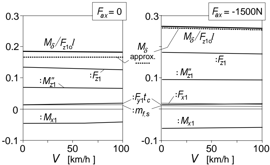
Fig. 10.21. The non-dimensional steer torque ( M_\delta/(F_{z10}l) ) and its components (cf. Eq.(10.147)) per m c.g. lateral offset y_{mr} . In M''_{z1} the F_{x1} contribution is removed.
