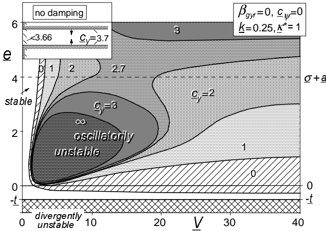
Fig. 6.6. Influence of lateral suspension compliance with non-dimensional stiffness c_y on stability. Gyroscopic couple and steer stiffness not regarded. Non-dimensional parameters: f = 0 , \underline{m} = 0.5 , \underline{t} = 0.5 , \underline{\sigma} = 3 .
