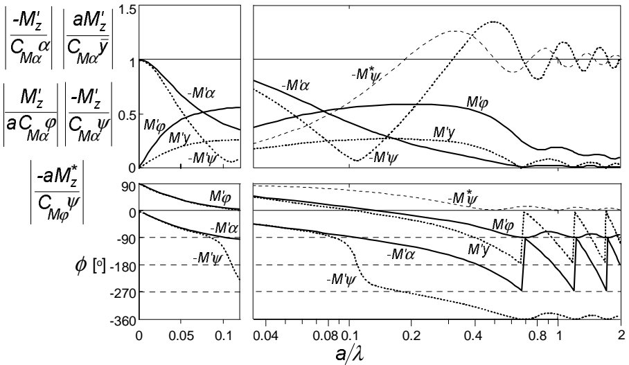
Fig. 5.34. Frequency response functions of string model with tread elements for the aligning torque with respect to various motion input variables. Same conditions as in Fig. 5.33. The response functions of the moment due to tread width M'_z have been added.
