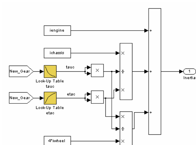
Figure 6.16: Inertia Evaluation Block.
