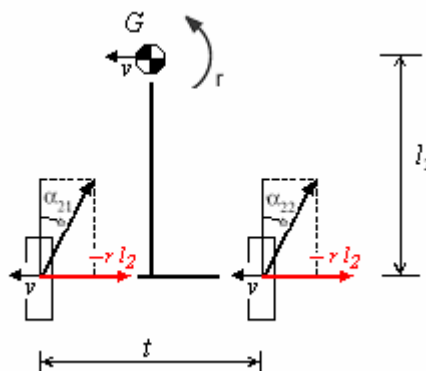
Figure 5.5: Lateral Components of Velocity at Rear Tyres
