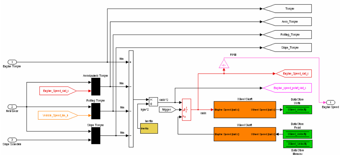
Figure 6.12: Driveline Subsystem.
