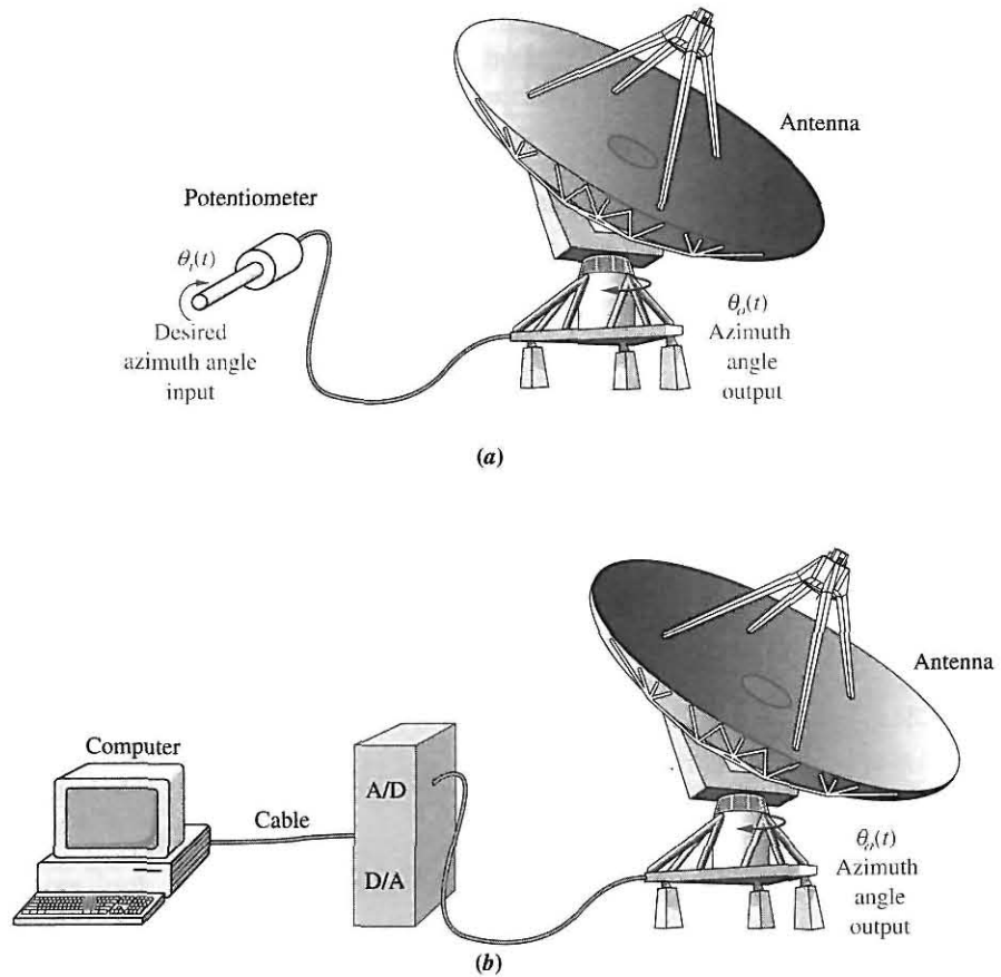
FIGURE 13.1 Conversion of antenna azimuth position control system from a. analog control to b. digital control
