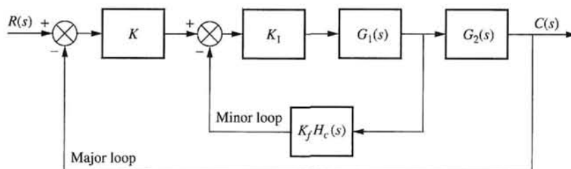
FIGURE 9.45 Generic control system with feedback compensation.
