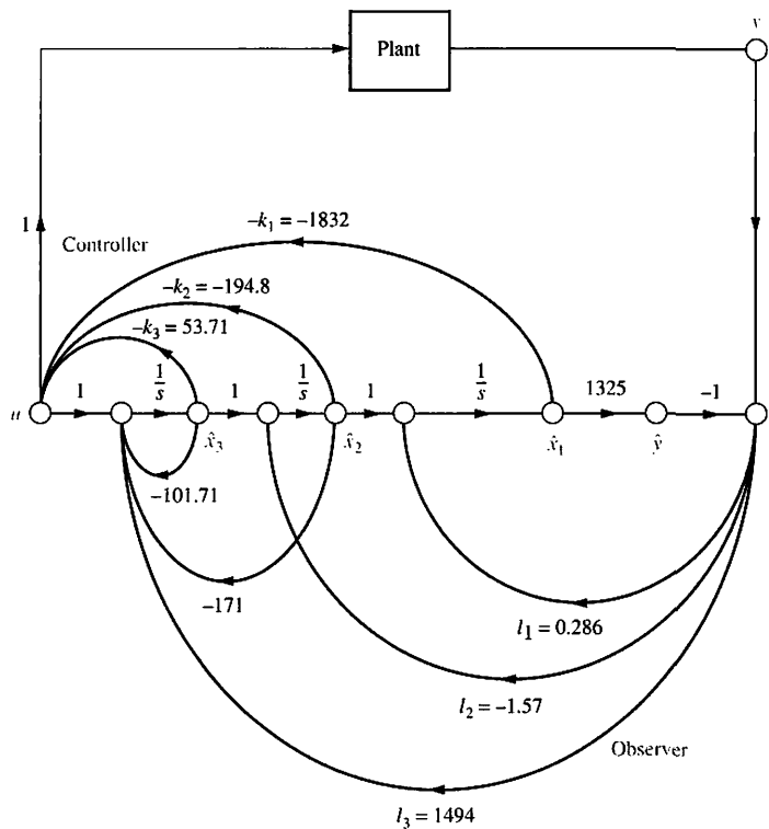
FIGURE 12.26 Completed state-space design for the antenna azimuth position control system, showing controller and observer
