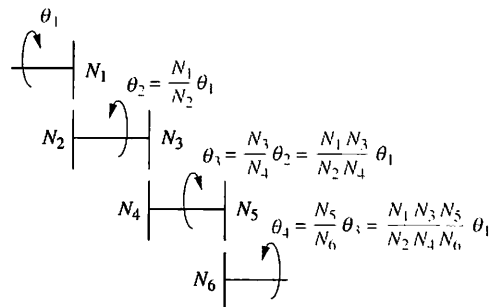
FIGURE 2.31 Gear train
