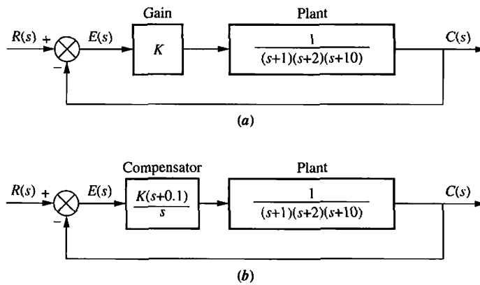
FIGURE 9.4 Closed-loop system for Example 9.1: a. before compensation; b. after ideal integral compensation
