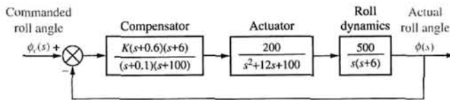
FIGURE P6.15 Towed vehicle roll control
