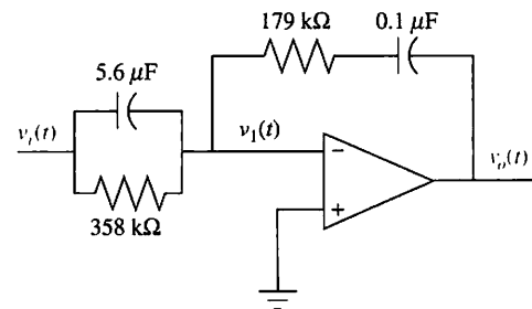
FIGURE 9.62 PID controller
