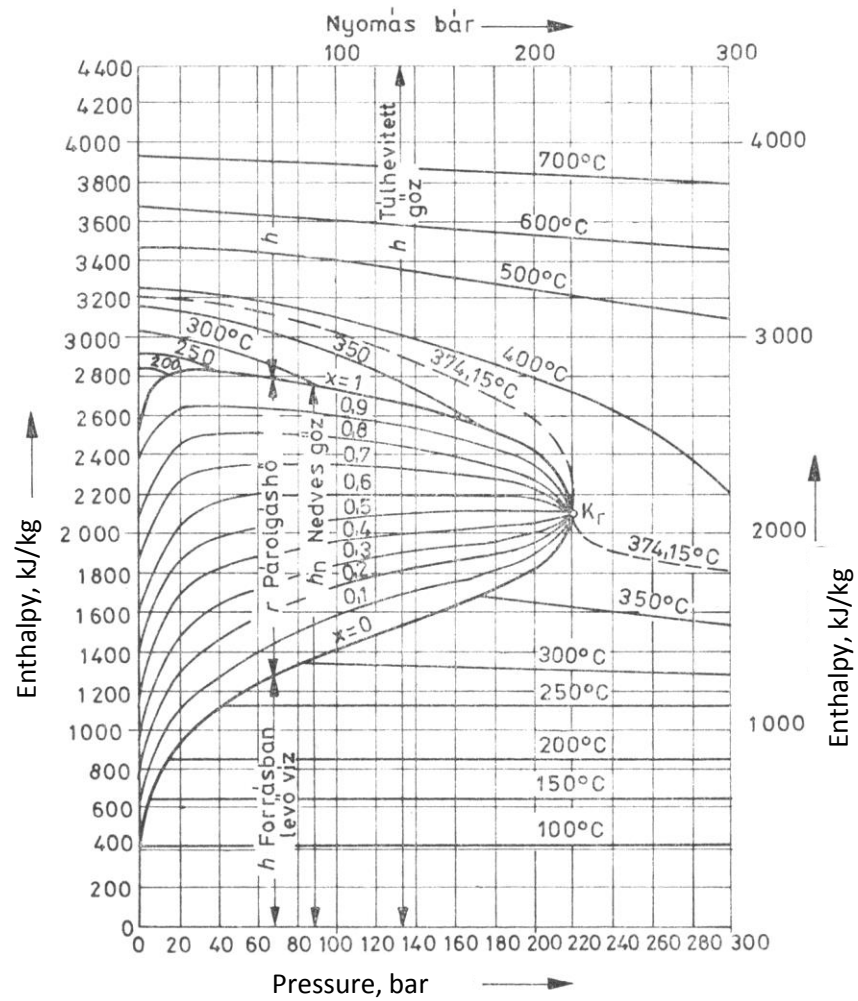
Water h-p chart
